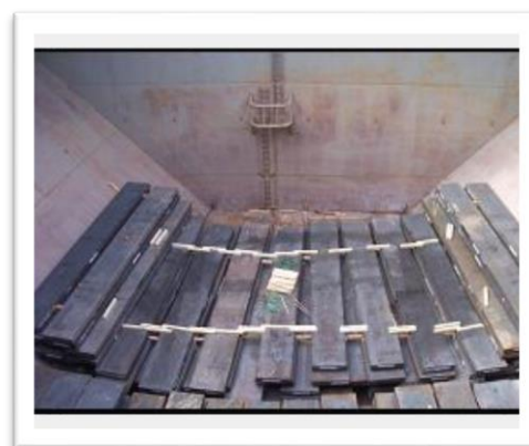
Steel Slabs in the Hold of a Bulk Carrier
